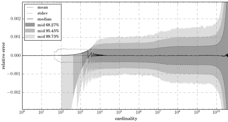
Figure 17: Relative error of the maximum likelihood estimates as a function of the true cardinality for a HyperLogLog sketch with parameters p = 22 and q = 10 .
